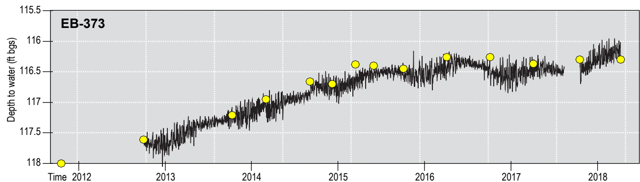
Figure 5. EB-373 is 300 feet deep, located near the Santa Fe airport, and completed in the Tesuque Formation.
